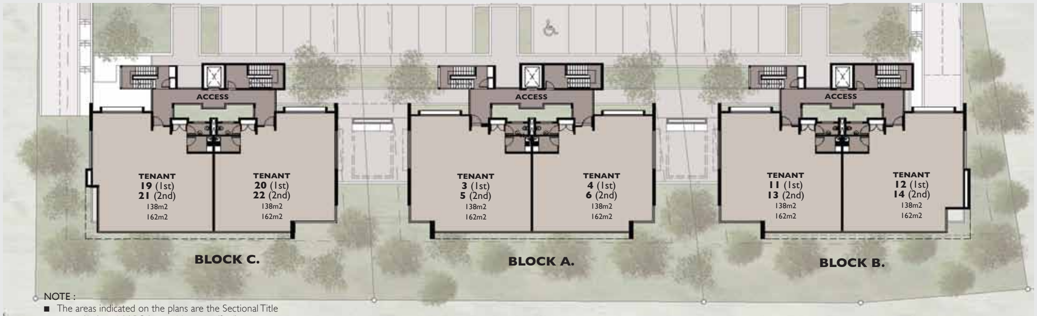
TYPICAL FIRST & SECOND FLOOR PLAN
